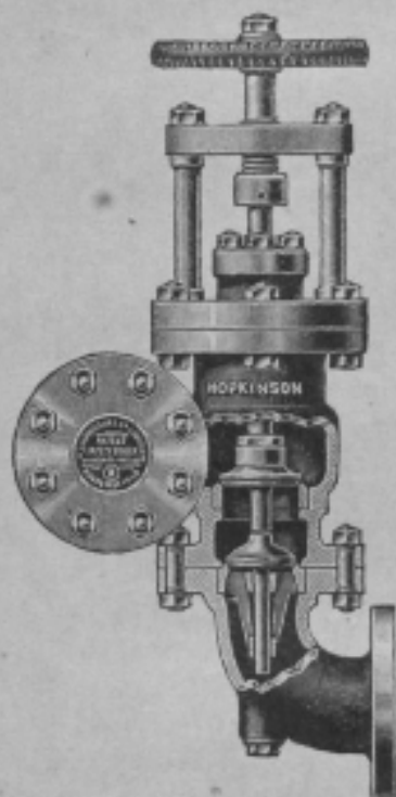
HOPKINSON'S PATENT "ACCESSIBLE" CHECK FEED VALVE FIG. 1320
